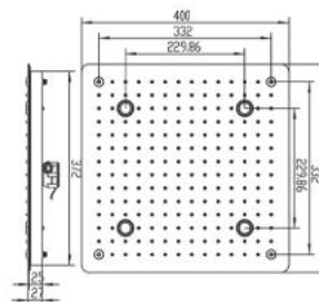
CELLING CR - SQ40GLED - ( 40 CM )
