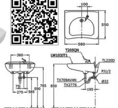
Wall Hung Lavatory 580W X 550D X 850H mm
