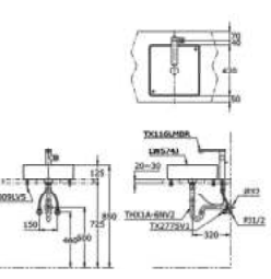
Console Lavatory 420W x 420D x 125H mm
